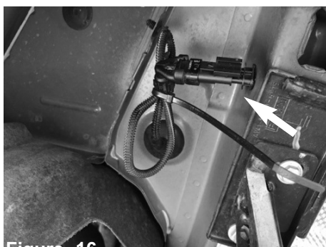
Figure 16 Now with provided Exhaust Valve by-pass module, connect to the harness from step 3. Tighten up and bundle the harness using provided zip-tie. Note: Make sure the Exhaust valve by-pass module is installed or vehicle will not be able to select Drive modes.
