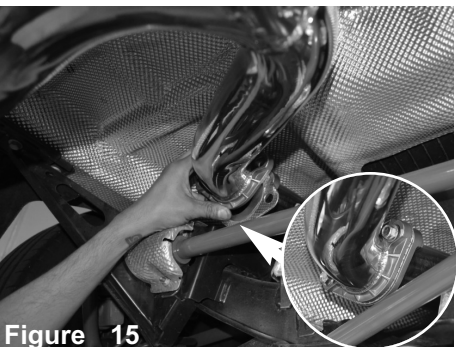
Figure 15 Secure flanges using provided gasket and M8 bolts and nuts. DO NOT TIGHTEN! Now position for the best fit. This may require to loosen and retighten other flanges. Tighten all flanges using 14mm socket and wrench. Secure and tighten band clamp. Push exhaust forward for exhaust to fit properly.
