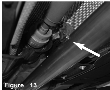
Figure 13 Verify the metal hangar has clearance and does not come close to the drive shaft.
