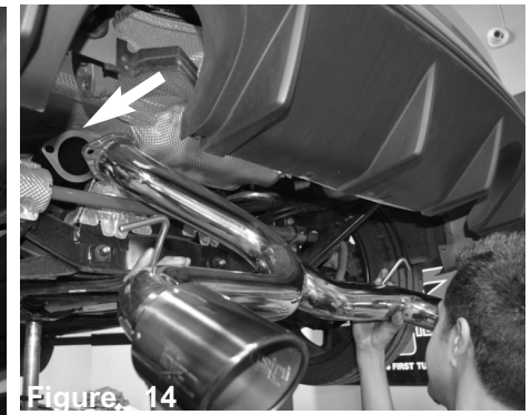
Figure 14 Install the rear piece into the vehicle. Position the flange. Position the hangars to the rubber isolator.
