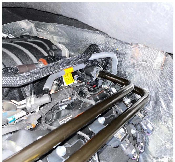
10. Connect the high pressure fuel supply line to the RH fuel rail and lock it into position.
