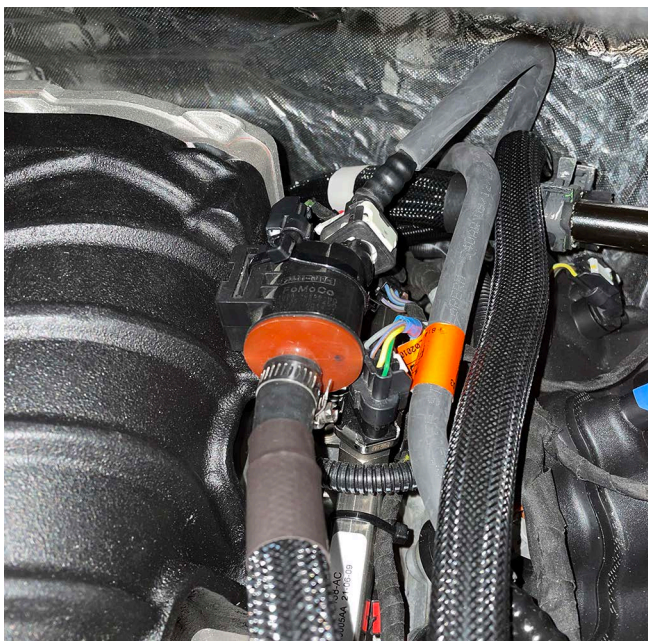
8. Install the fuel inlet line to the tube on the LH fuel
