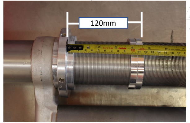
Set the preload collar all the way up to the Resi bridge and the crossover ring to 120mm from the spring seat to the bottom of the crossover ring.
