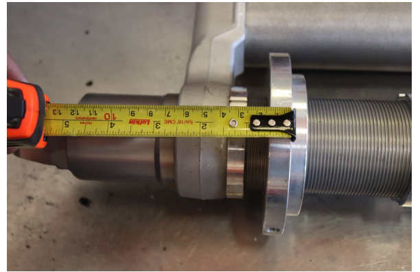
Set the preload collar to 35mm from the bottom of the Resi crossover to the bottom of the preload collar
