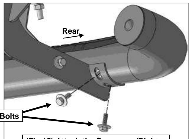
(Fig 15) Attach the Passenger/Right Sidebar to the Rear Mounting Bracket
