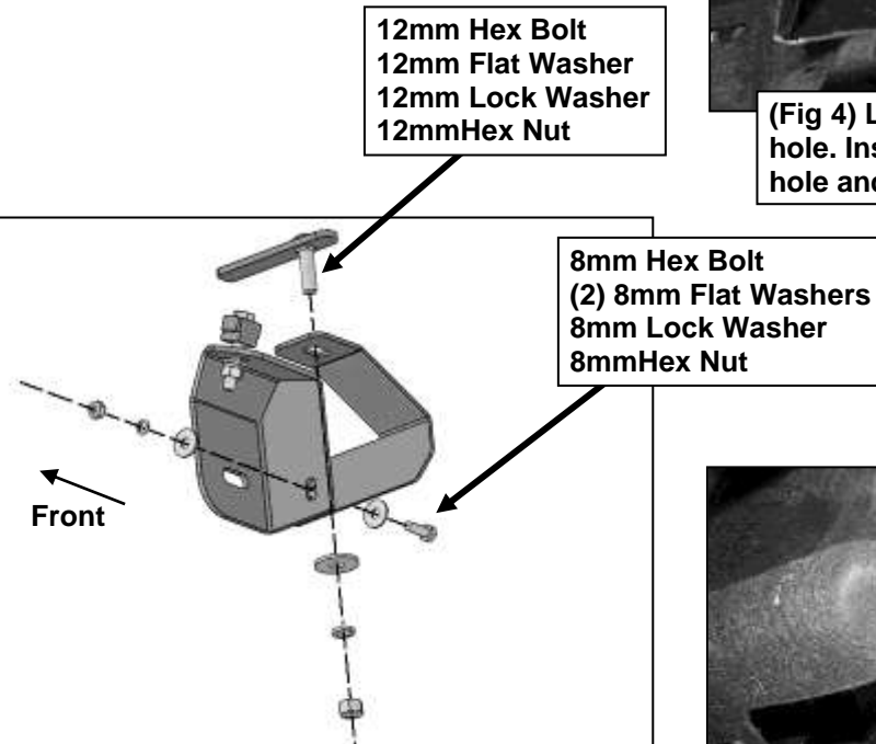
(Fig 5) Attach Passenger/Right Front Support Bracket to the Bolt Plate and the Mounting Bracket
