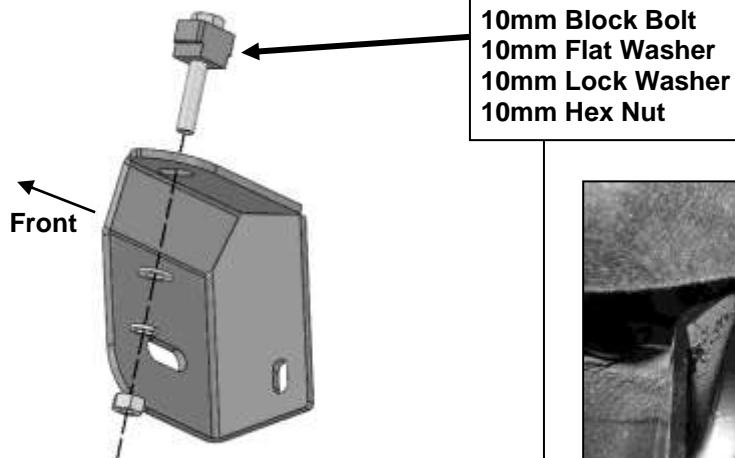
(Fig 3) Attach the Passenger/Right Front Mounting Bracket to the 10mm Block Bolt
