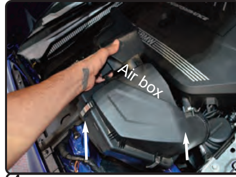
4. Carefully lift up and remove the airbox from the vehicle. Note: Next photo intake tube was removed for easier look at intake tube and for photos.
