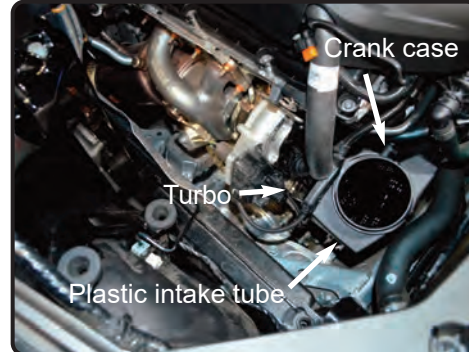
8. Re-install the plastic intake tube into the vehicle. Re-connect Crank case line. Make sure you hear a click, tug on tube to make sure the tube is secured to turbo and will not come off.
