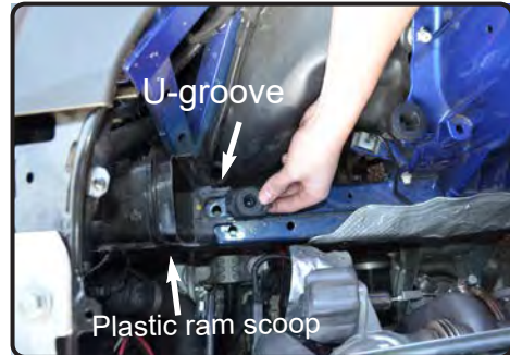
11. Remove the Air box grommet located on the frame in front of Plastic ram scoop. Heat shield will seat inside this plastic U-groove.
