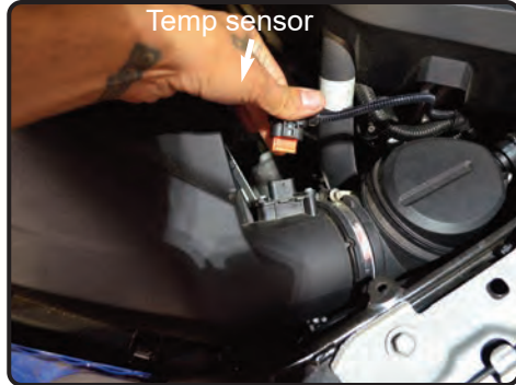
2. Disconnect the Temp sensor harness and pull harness cable from the air box.
